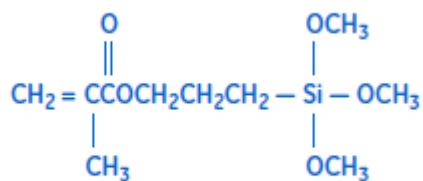
Gamma-Methacryloxypropyltrimethoxy Silane
