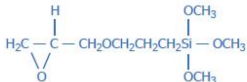
Gamma-Glycidoxypropyltrimethoxysilane
