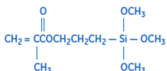
Gamma-Methacryloxypropyltrimethoxy Silane
