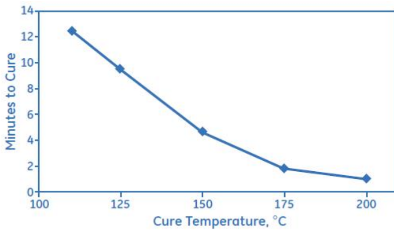
Figure 1: Addisil 6101 Silicone Adhesive Cure Time vs Temperature
