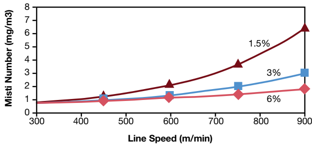
Figure 3. SilForce SL6425 misting characteristics at various SLAM 3000 silicone anti-mist additive concentrations and various machine speeds
