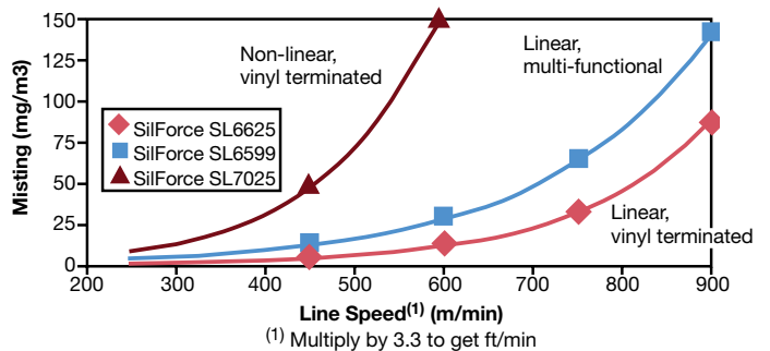
Figure 1. Misting properties of various silicone polymers at constant viscosity and equal coating parameters Lower viscosity vinyl polymers will typically generate less mist than higher viscosity coatings as illustrated in Figure 2.
