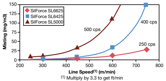
Figure 2. Misting properties of vinyl terminated polymers at various viscosities
