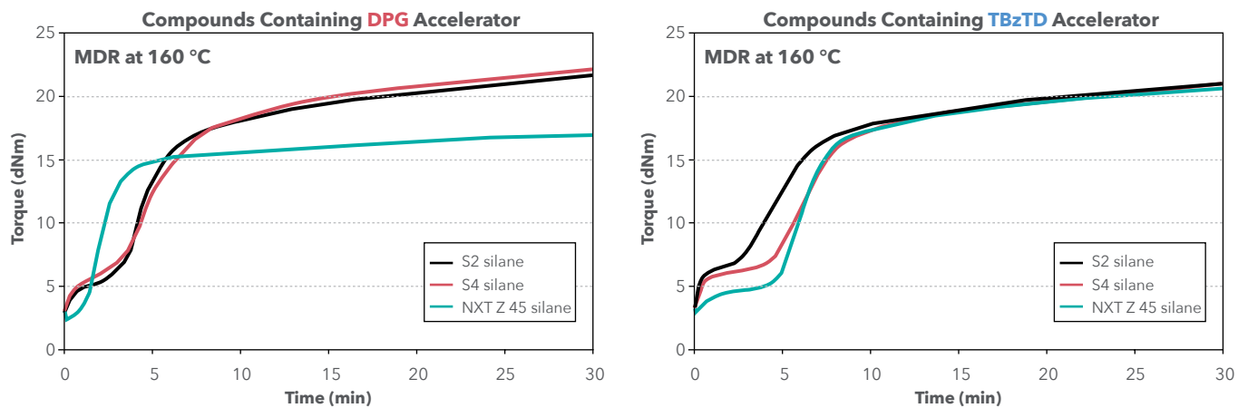
Figure 1: Cure Curve Comparison of S2 (TESPD) Silane, S4 (TESPT) Silane, and NXT Z 45 Silane in Rubber Compounds
