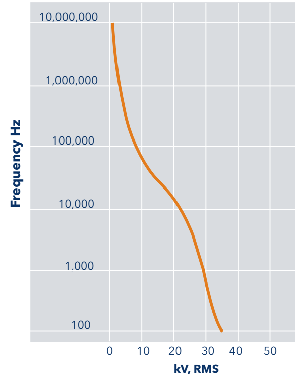
Representative values of the dielectric breakdown voltage of fused quartz, 0.75 mm thick samples. Source: Momentive*
