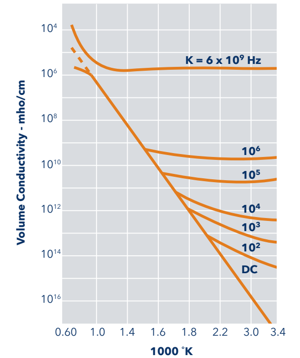
Volume conductivity of fused quartz. Source: Momentive*
