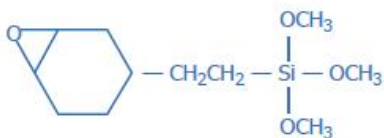
Beta-(3,4-Epoxy)cyclohexyl ethyltrimethoxysilane
